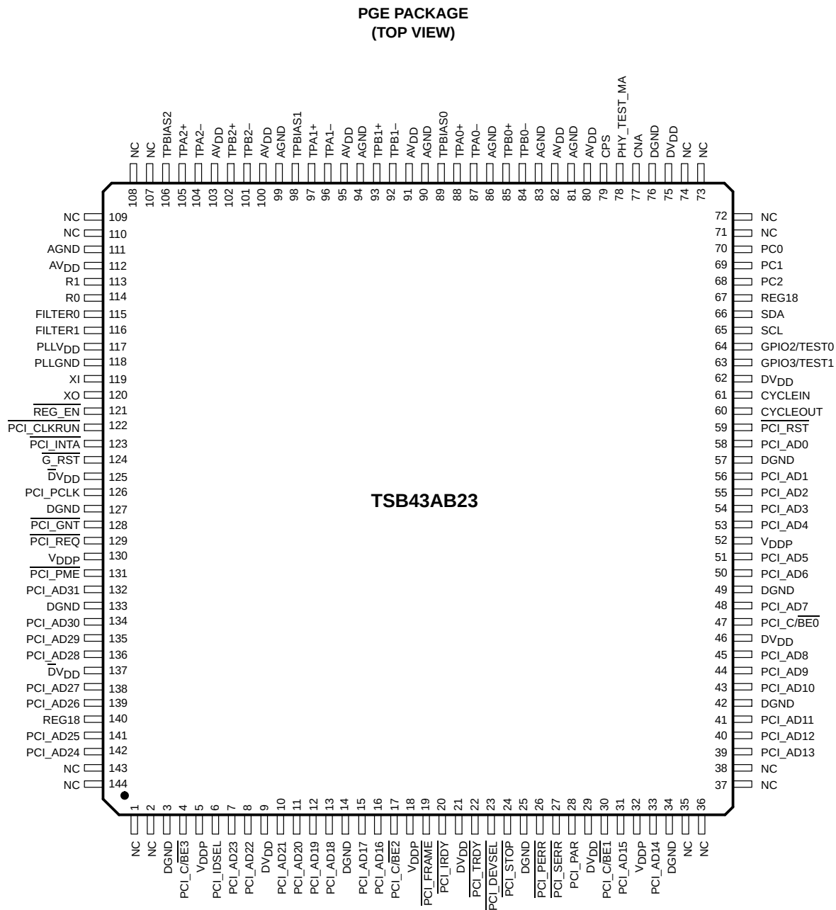
Figure 2–2. PGE Package Terminal Assignments
