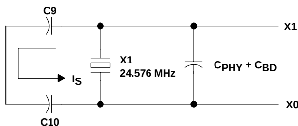
Figure 8–4. Load Capacitance for the TSB43AB23 PHY
